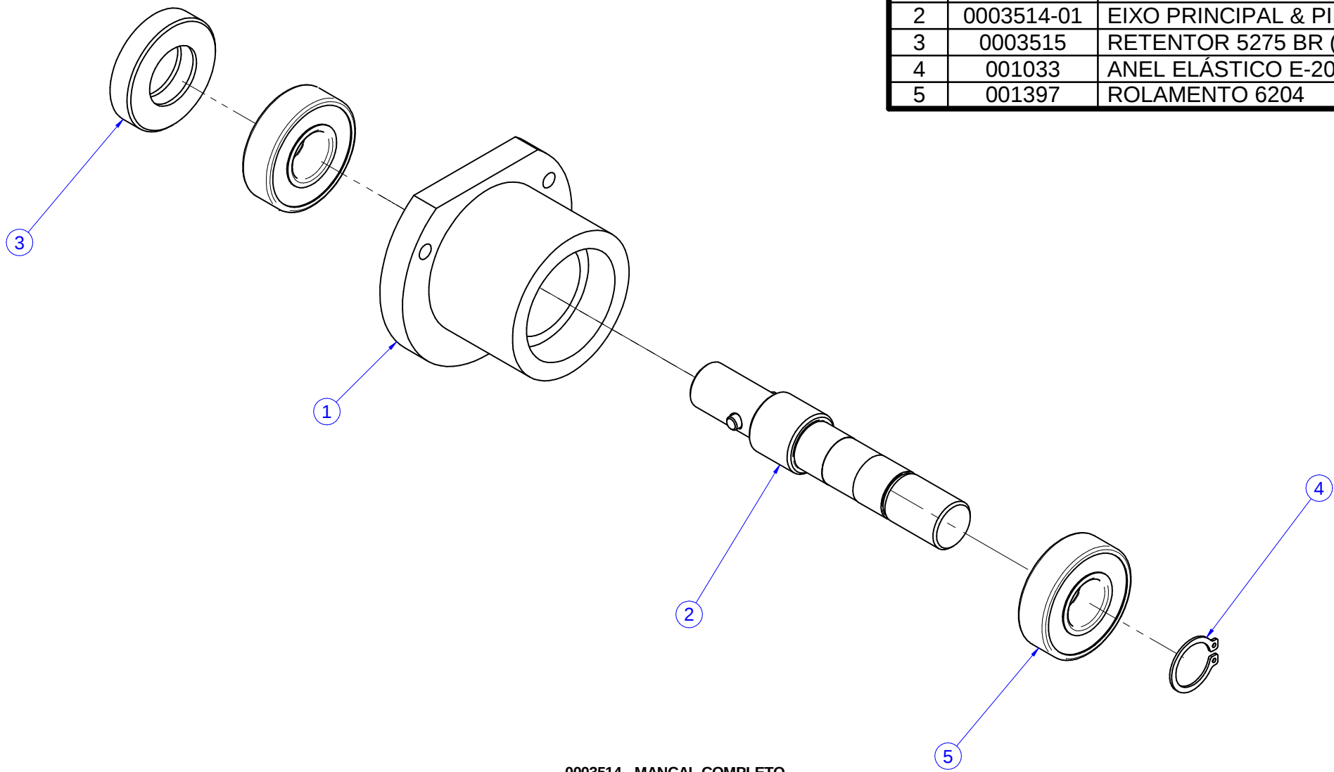
0003514 - MANCAL COMPLETO
