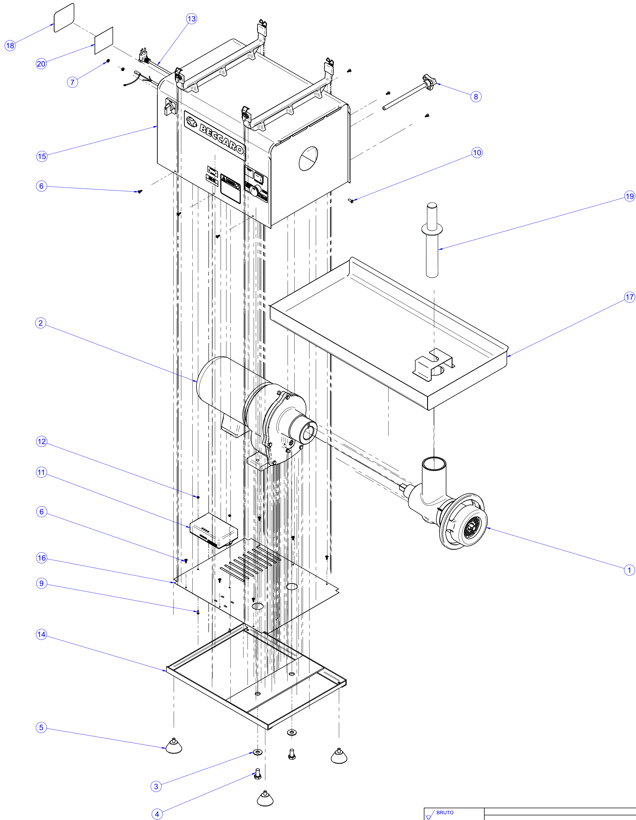
VISTA EXPLODIDA
